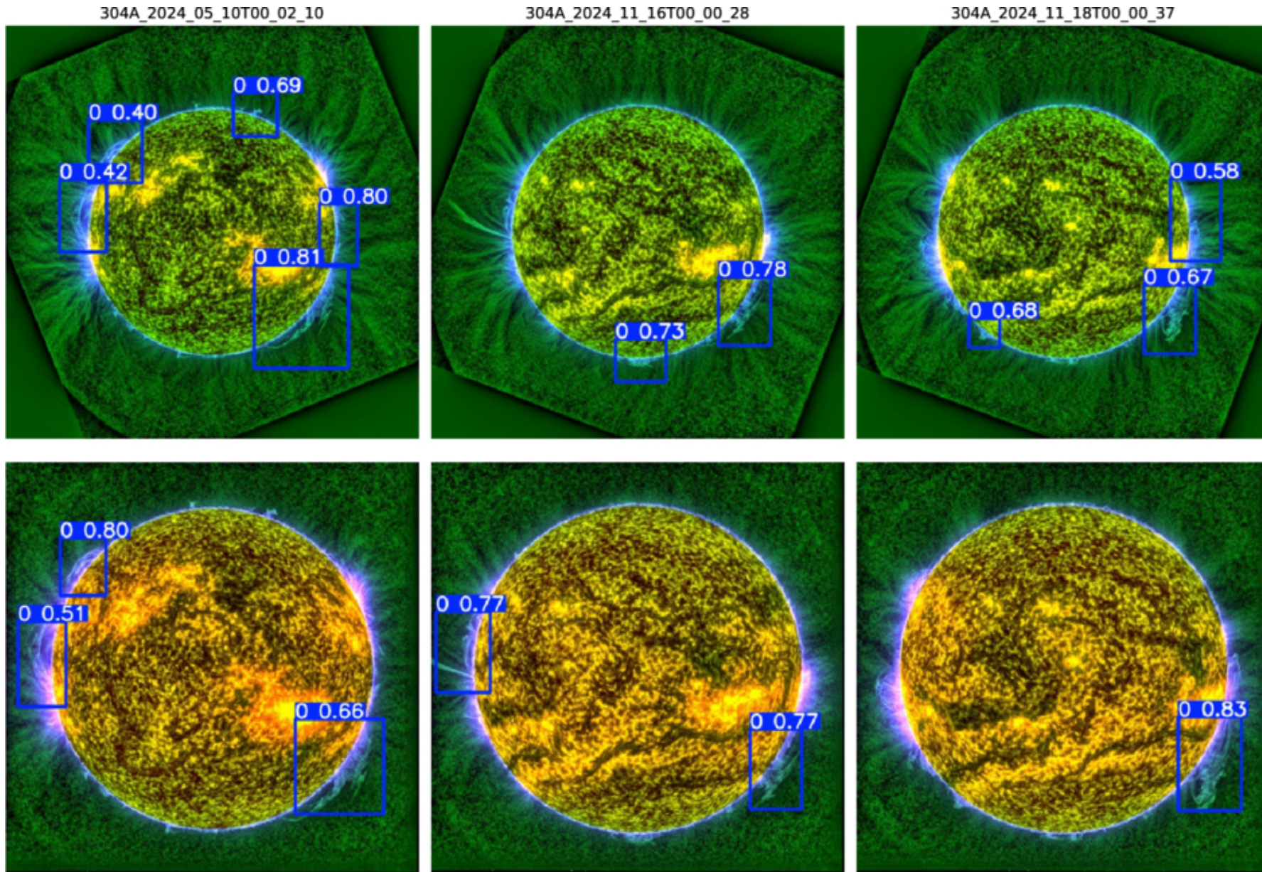
Figure 5. from Harry Birch et al 2026 Astrophys. J. 1003 doi:10.3847/1538-4357/ae664d https://dx.doi.org/10.3847/1538-4357/ae664d © 2026. The Author(s). Published by the American Astronomical Society.
