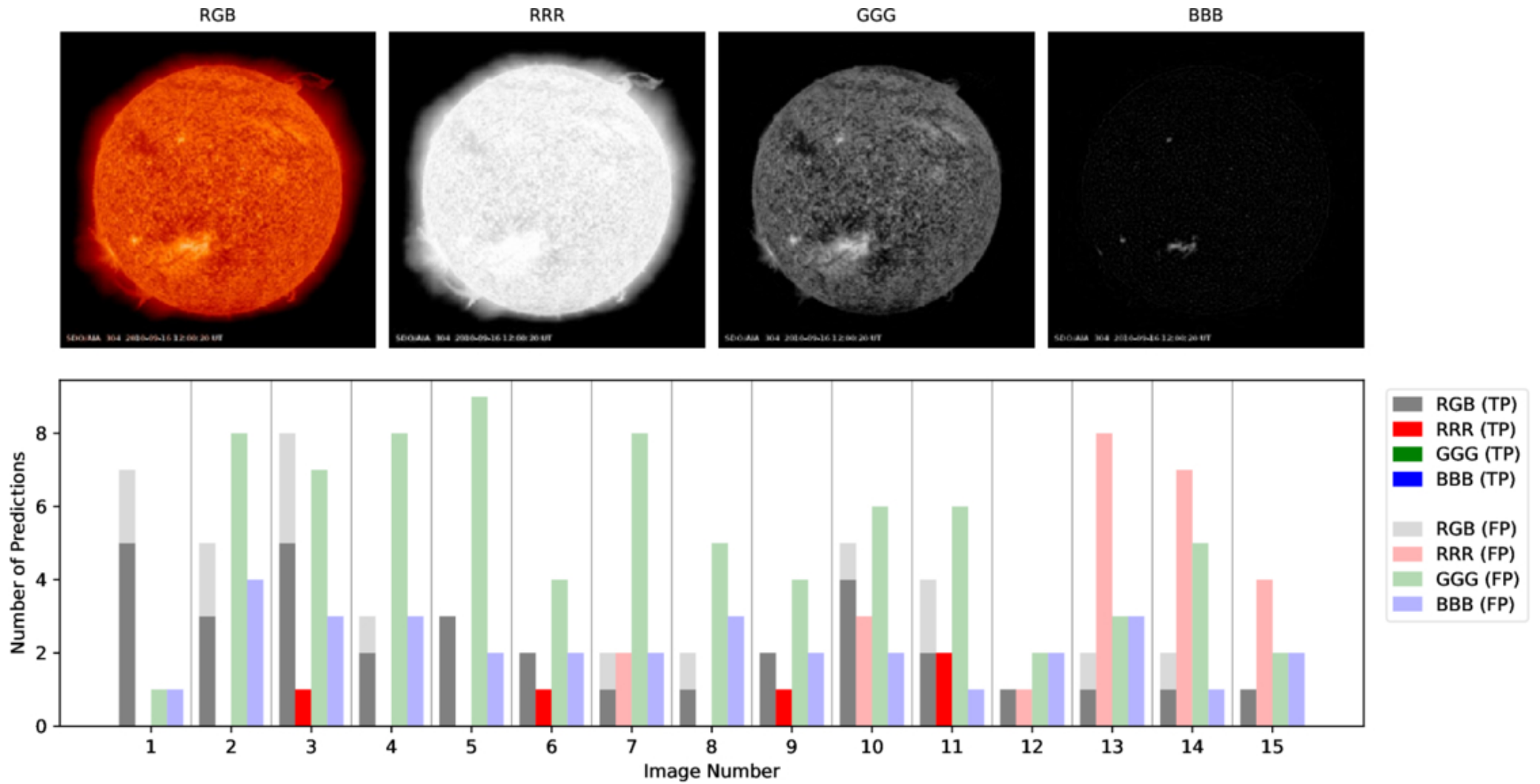
Figure 2. from Harry Birch et al 2026 Astrophys. J. 1003 doi:10.3847/1538-4357/ae664d https://dx.doi.org/10.3847/1538-4357/ae664d © 2026. The Author(s). Published by the American Astronomical Society.
