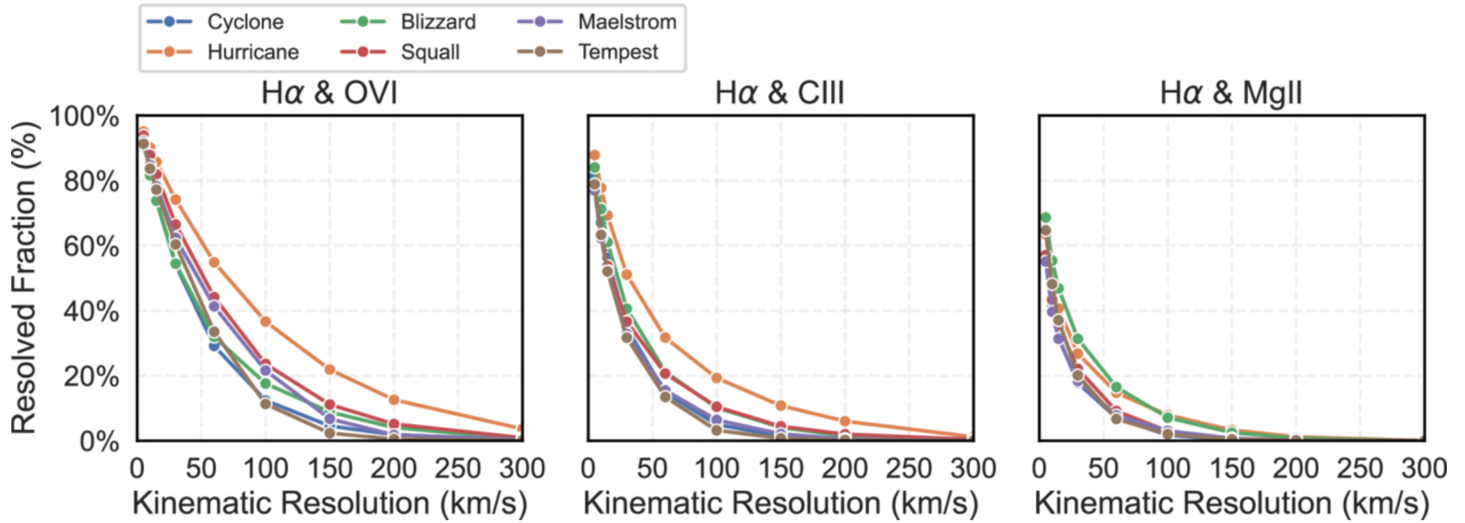
Figure 9. from Vida Saeedzadeh et al 2026 Astrophys. J. 1004 doi:10.3847/1538-4357/ae658a https://dx.doi.org/10.3847/1538-4357/ae658a © 2026. The Author(s). Published by the American Astronomical Society.
