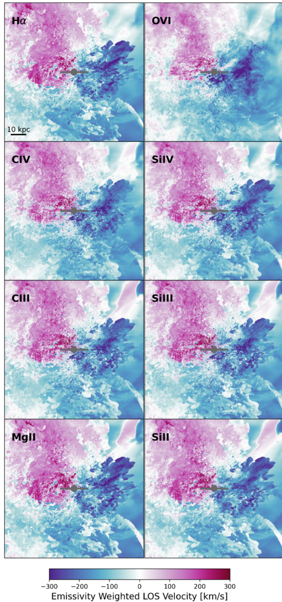
Figure 7. from Vida Saeedzadeh et al 2026 Astrophys. J. 1004 doi:10.3847/1538-4357/ae658a https://dx.doi.org/10.3847/1538-4357/ae658a © 2026. The Author(s). Published by the American Astronomical Society.
