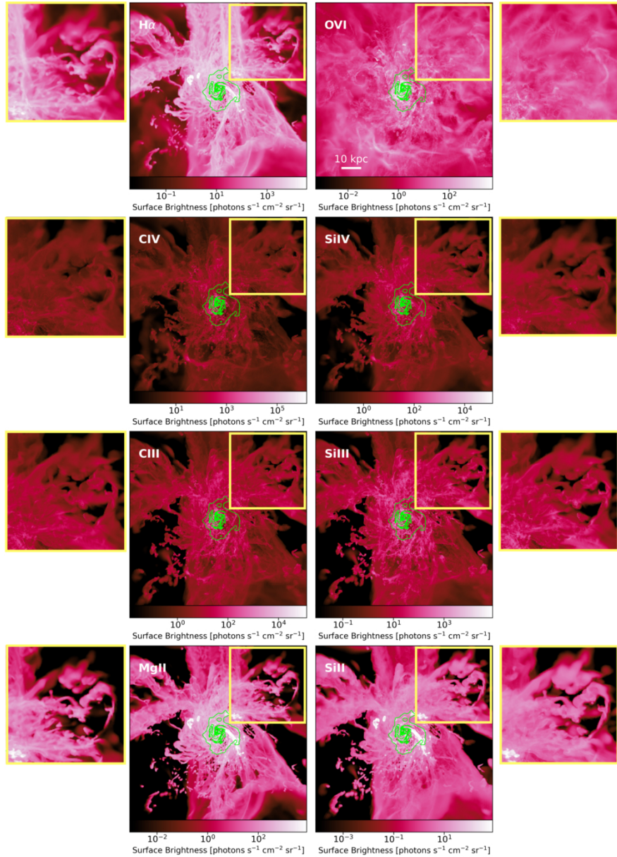
Figure 2. from Vida Saeedzadeh et al 2026 Astrophys. J. 1004 doi:10.3847/1538-4357/ae658a https://dx.doi.org/10.3847/1538-4357/ae658a © 2026. The Author(s). Published by the American Astronomical Society.
