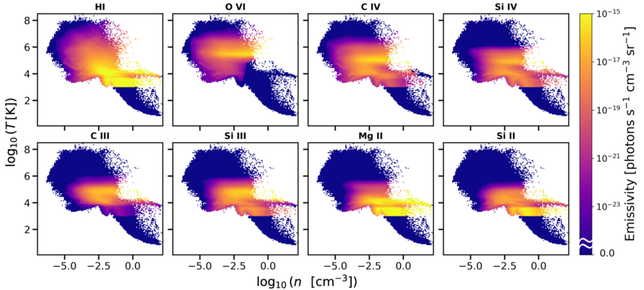
Figure 17. from Vida Saeedzadeh et al 2026 Astrophys. J. 1004 doi:10.3847/1538-4357/ae658a https://dx.doi.org/10.3847/1538-4357/ae658a © 2026. The Author(s). Published by the American Astronomical Society.
