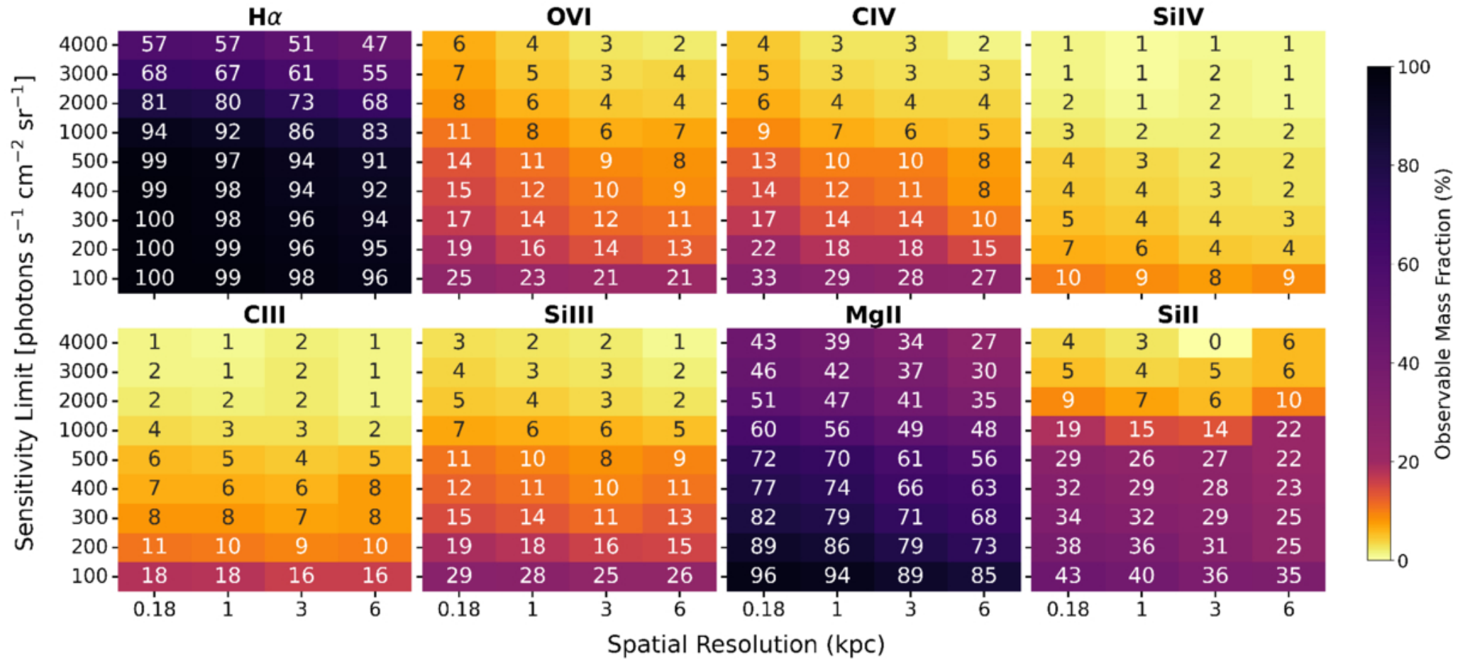
Figure 15. from Vida Saeedzadeh et al 2026 Astrophys. J. 1004 doi:10.3847/1538-4357/ae658a https://dx.doi.org/10.3847/1538-4357/ae658a © 2026. The Author(s). Published by the American Astronomical Society.
