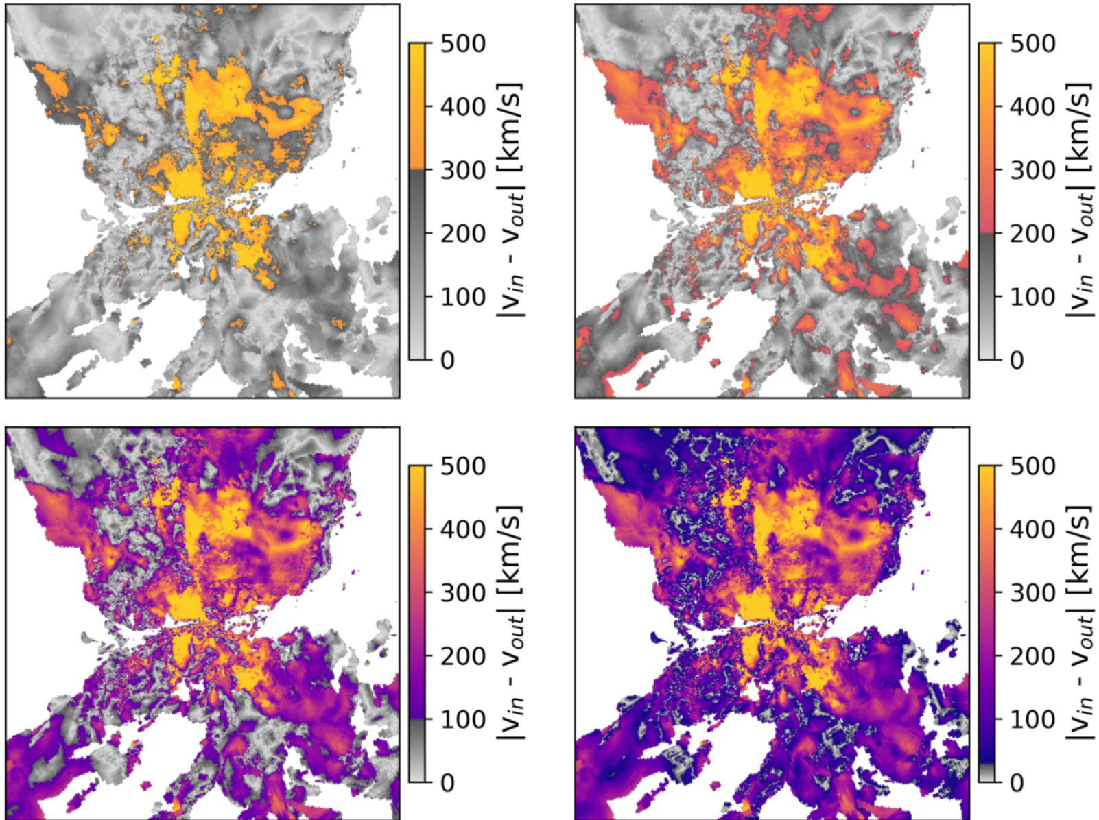
Figure 11. from Vida Saeedzadeh et al 2026 Astrophys. J. 1004 doi:10.3847/1538-4357/ae658a https://dx.doi.org/10.3847/1538-4357/ae658a © 2026. The Author(s). Published by the American Astronomical Society.
