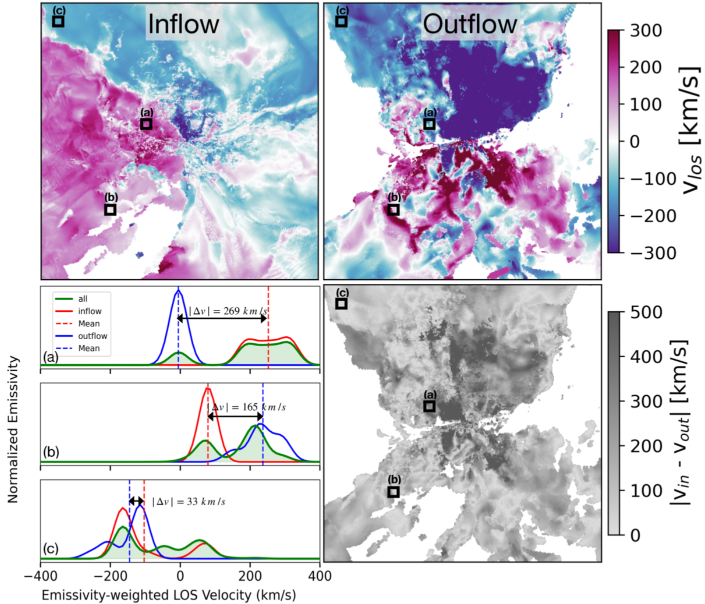
Figure 10. from Vida Saeedzadeh et al 2026 Astrophys. J. 1004 doi:10.3847/1538-4357/ae658a https://dx.doi.org/10.3847/1538-4357/ae658a © 2026. The Author(s). Published by the American Astronomical Society.
