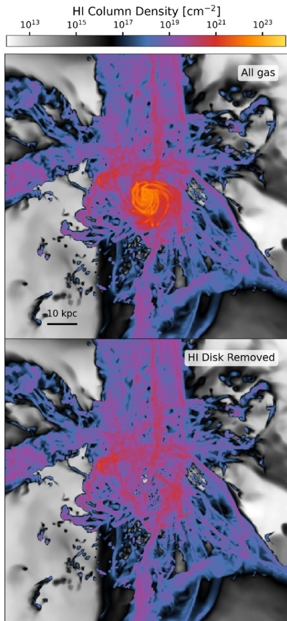
Figure 1. from Vida Saeedzadeh et al 2026 Astrophys. J. 1004 doi:10.3847/1538-4357/ae658a https://dx.doi.org/10.3847/1538-4357/ae658a © 2026. The Author(s). Published by the American Astronomical Society.
