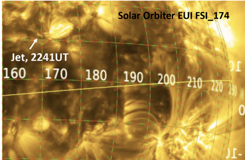
Figure 7. from D. G. Mitchell et al 2026 Astrophys. J. 1003 doi:10.3847/1538-4357/ae6589 https://dx.doi.org/10.3847/1538-4357/ae6589 © 2026. The Author(s). Published by the American Astronomical Society.
