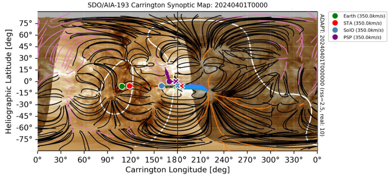
Figure 10. from D. G. Mitchell et al 2026 Astrophys. J. 1003 doi:10.3847/1538-4357/ae6589 https://dx.doi.org/10.3847/1538-4357/ae6589 © 2026. The Author(s). Published by the American Astronomical Society.
