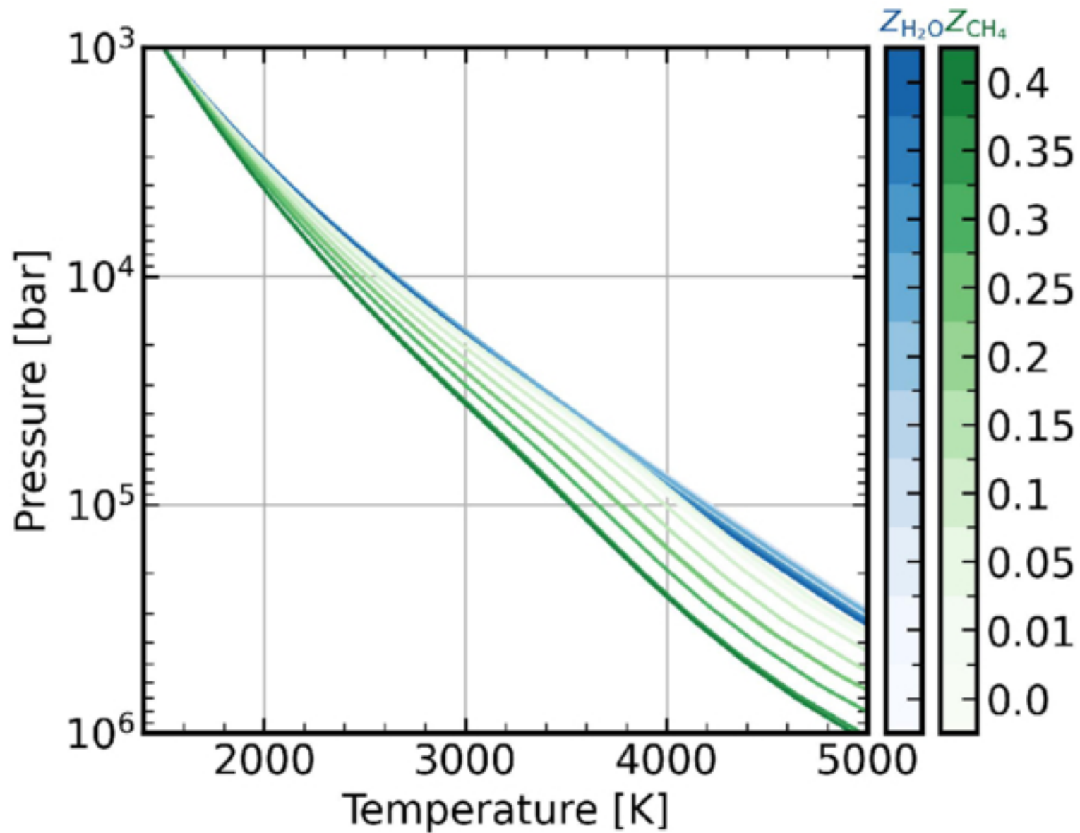
Figure 8. from Caroline Piaulet-Ghorayeb et al 2026 Astrophys. J. 1006 doi:10.3847/1538-4357/ae64ff https://dx.doi.org/10.3847/1538-4357/ae64ff © 2026. The Author(s). Published by the American Astronomical Society.
