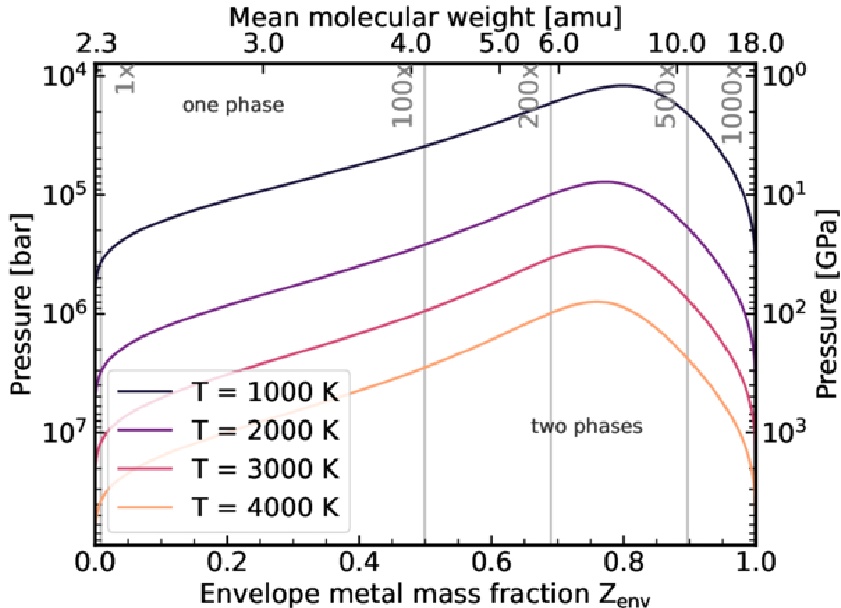
Figure 6. from Caroline Piaulet-Ghorayeb et al 2026 Astrophys. J. 1006 doi:10.3847/1538-4357/ae64ff https://dx.doi.org/10.3847/1538-4357/ae64ff © 2026. The Author(s). Published by the American Astronomical Society.
