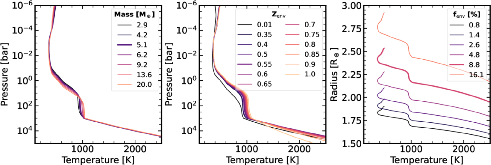
Figure 4. from Caroline Piaulet-Ghorayeb et al 2026 Astrophys. J. 1006 doi:10.3847/1538-4357/ae64ff https://dx.doi.org/10.3847/1538-4357/ae64ff © 2026. The Author(s). Published by the American Astronomical Society.
