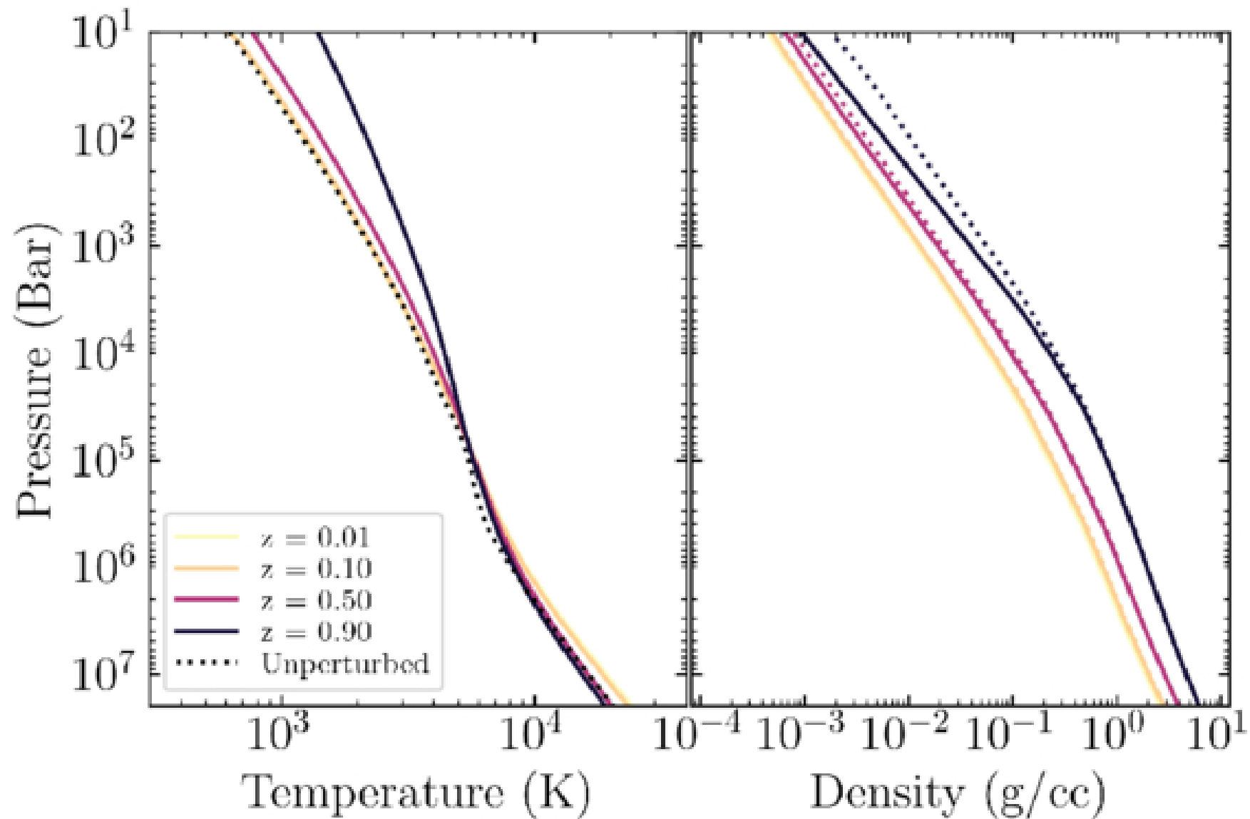
Figure 3. from Caroline Piaulet-Ghorayeb et al 2026 Astrophys. J. 1006 doi:10.3847/1538-4357/ae64ff https://dx.doi.org/10.3847/1538-4357/ae64ff © 2026. The Author(s). Published by the American Astronomical Society.
