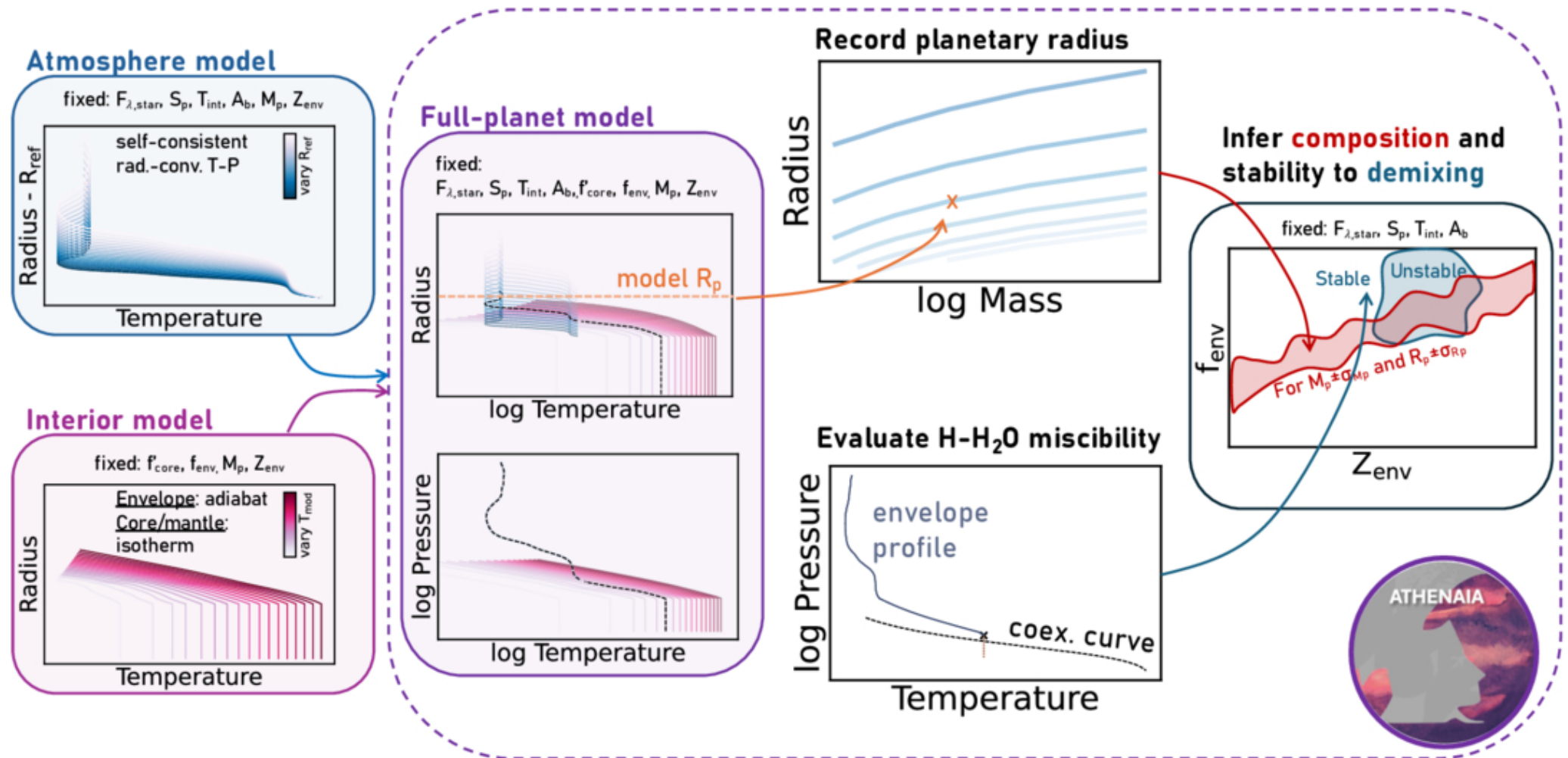
Figure 2. from Caroline Piaulet-Ghorayeb et al 2026 Astrophys. J. 1006 doi:10.3847/1538-4357/ae64ff https://dx.doi.org/10.3847/1538-4357/ae64ff © 2026. The Author(s). Published by the American Astronomical Society.
