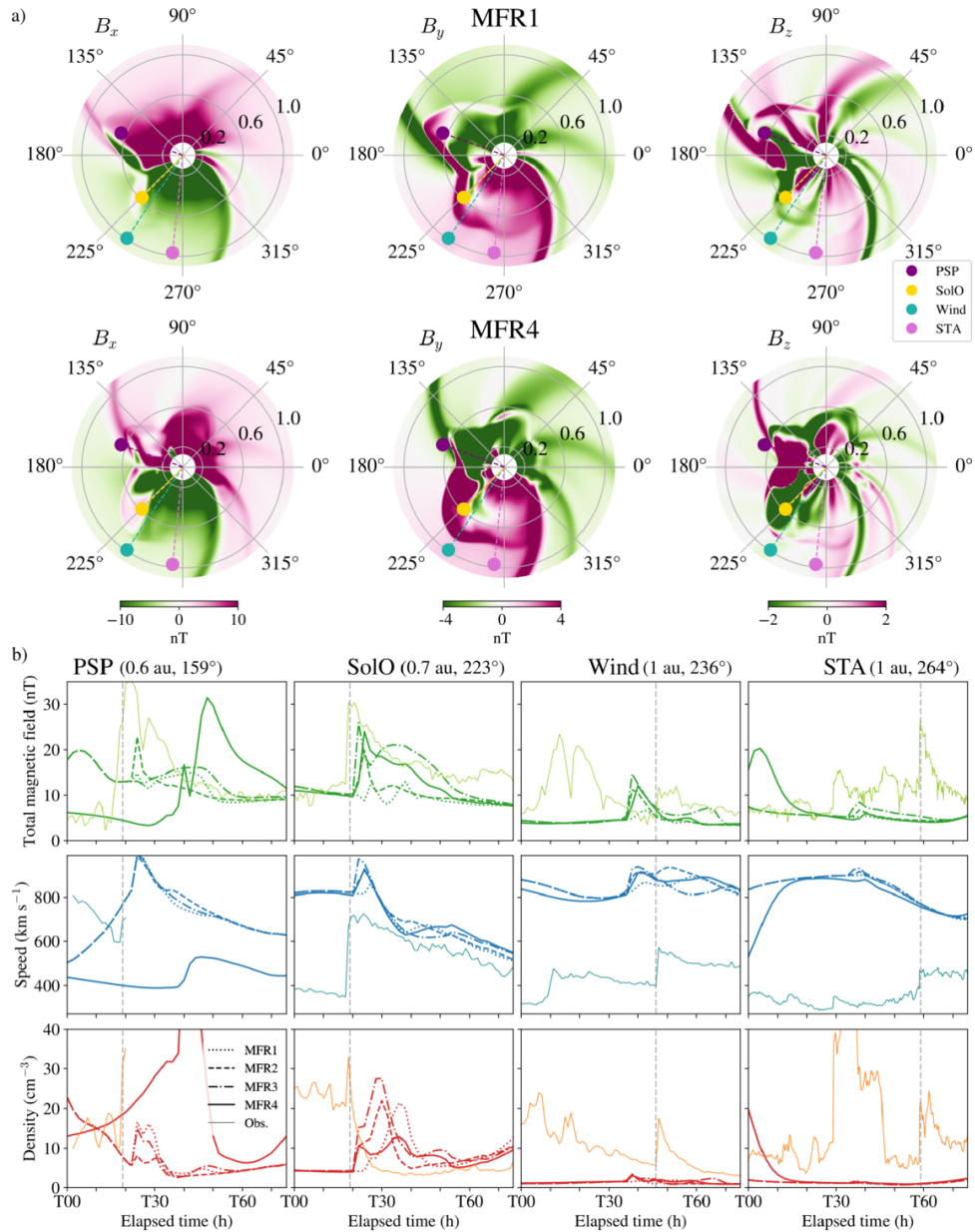
Figure 7. from Abril Sahade et al 2026 Astrophys. J. 1003 doi:10.3847/1538-4357/ae64f9 https://dx.doi.org/10.3847/1538-4357/ae64f9 © 2026. The Author(s). Published by the American Astronomical Society.
