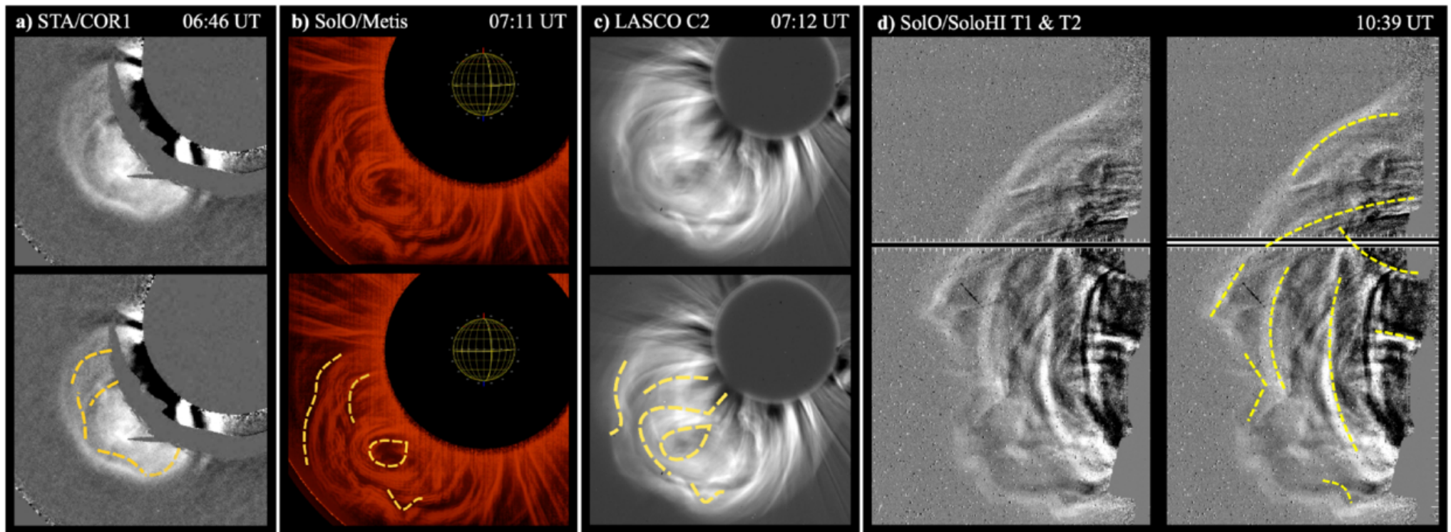
Figure 2. from Abril Sahade et al 2026 Astrophys. J. 1003 doi:10.3847/1538-4357/ae64f9 https://dx.doi.org/10.3847/1538-4357/ae64f9 © 2026. The Author(s). Published by the American Astronomical Society.
