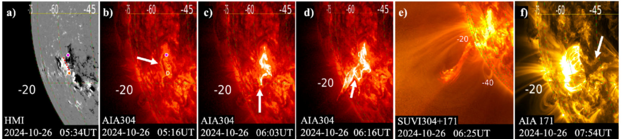
Figure 1. from Abril Sahade et al 2026 Astrophys. J. 1003 doi:10.3847/1538-4357/ae64f9 https://dx.doi.org/10.3847/1538-4357/ae64f9 © 2026. The Author(s). Published by the American Astronomical Society.
