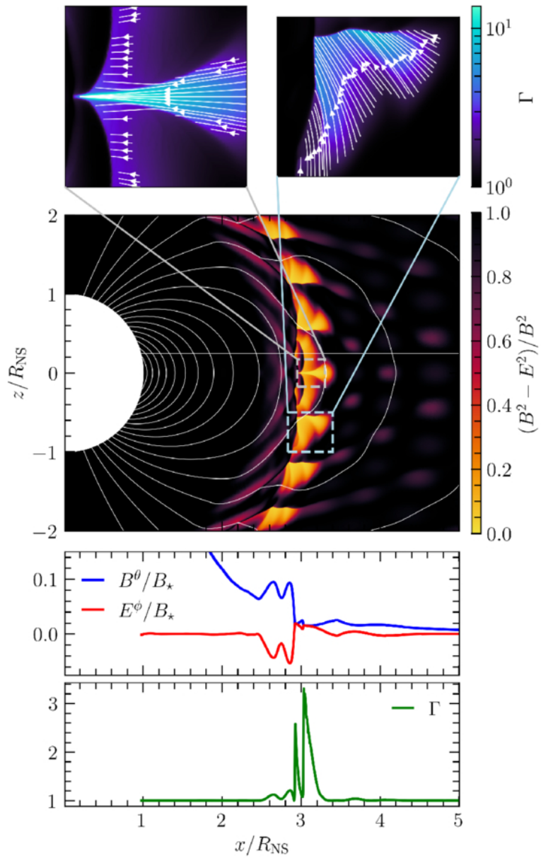
Figure 8. from Michael P. Grehan et al 2026 Astrophys. J. 1005 doi:10.3847/1538-4357/ae633a https://dx.doi.org/10.3847/1538-4357/ae633a © 2026. The Author(s). Published by the American Astronomical Society.
