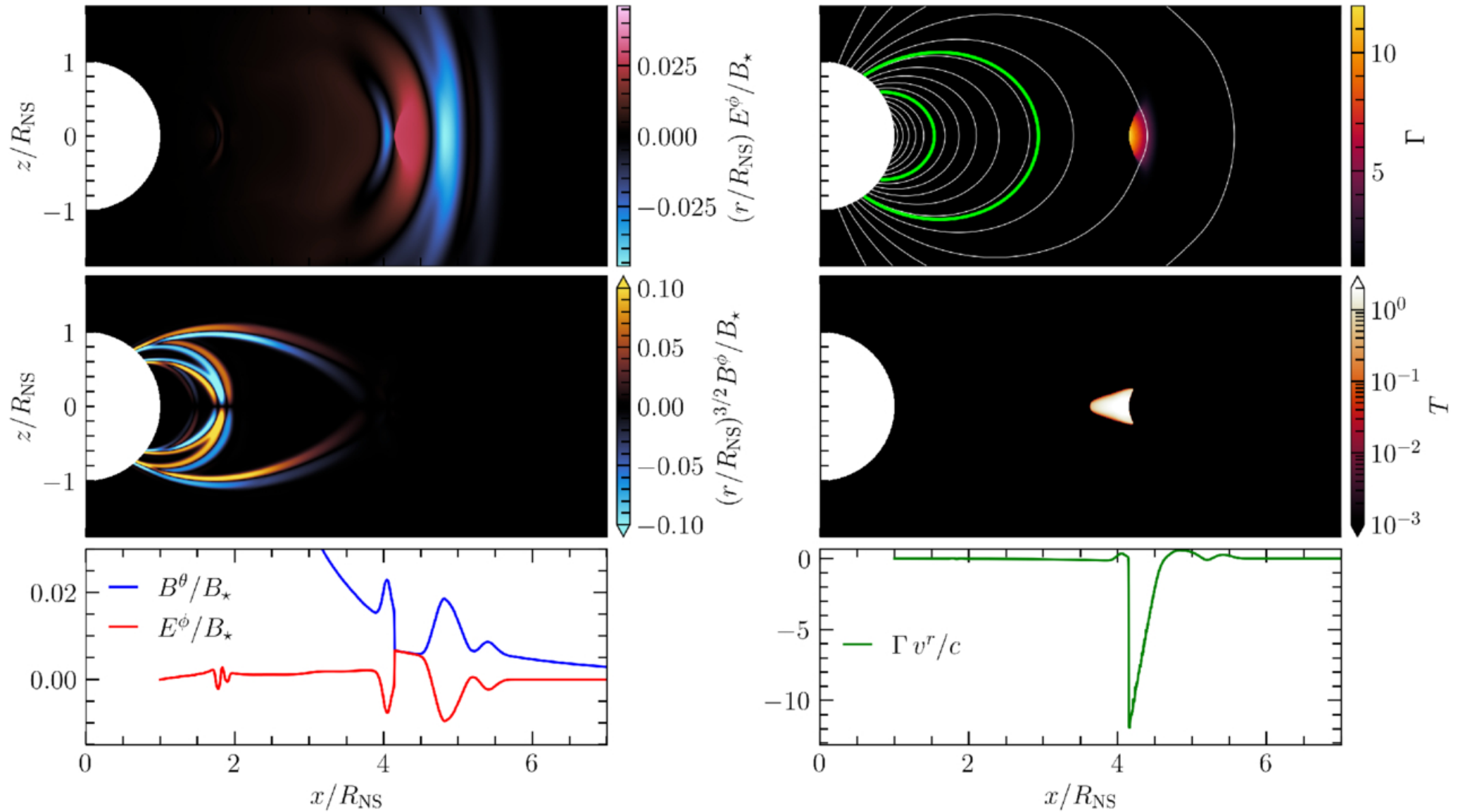
Figure 7. from Michael P. Grehan et al 2026 Astrophys. J. 1005 doi:10.3847/1538-4357/ae633a https://dx.doi.org/10.3847/1538-4357/ae633a © 2026. The Author(s). Published by the American Astronomical Society.
