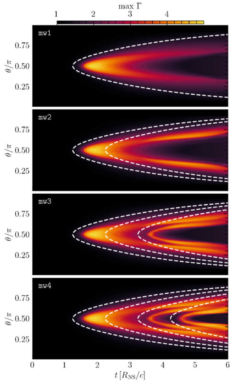
Figure 5. from Michael P. Grehan et al 2026 Astrophys. J. 1005 doi:10.3847/1538-4357/ae633a https://dx.doi.org/10.3847/1538-4357/ae633a © 2026. The Author(s). Published by the American Astronomical Society.
