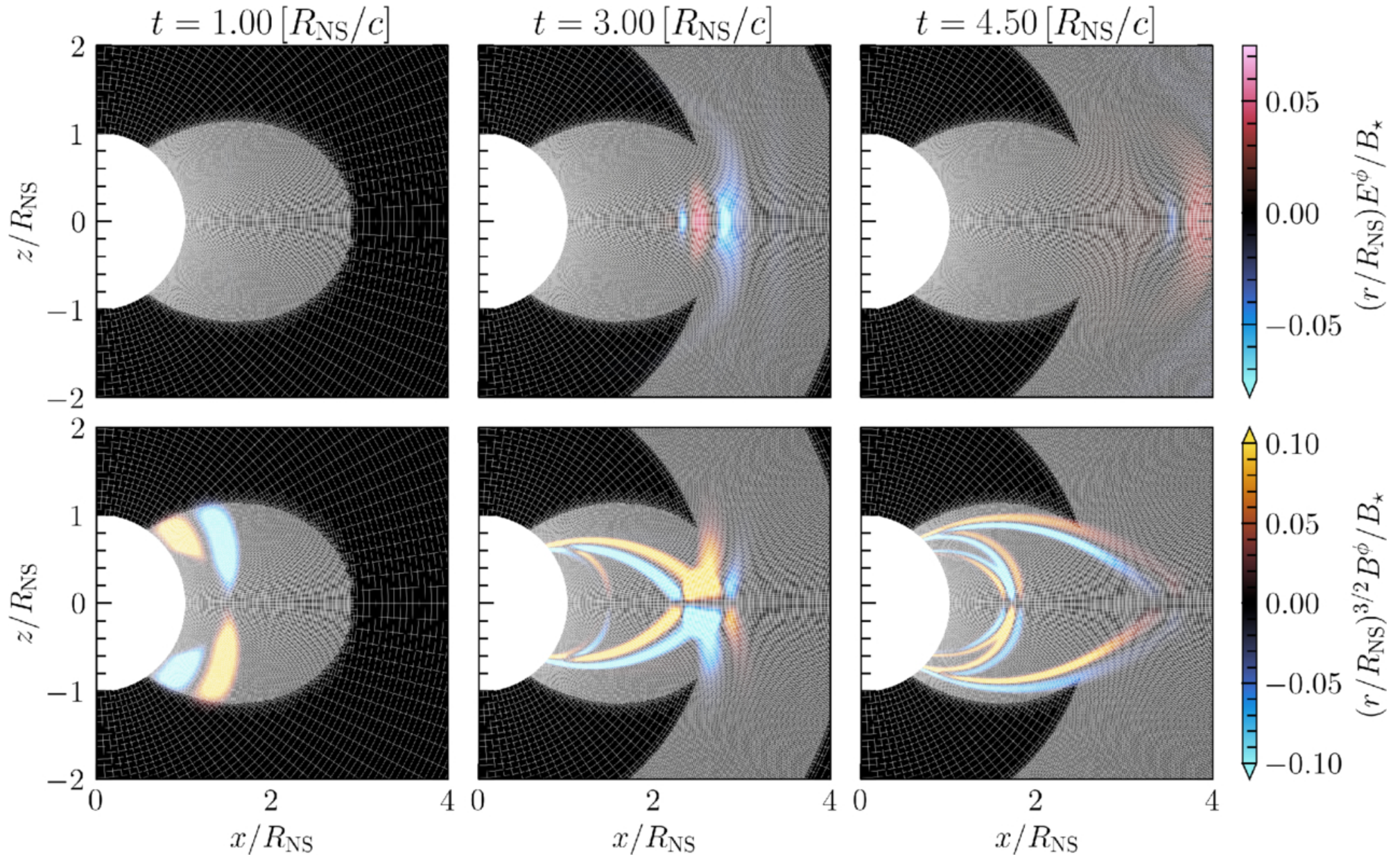
Figure 12. from Michael P. Grehan et al 2026 Astrophys. J. 1005 doi:10.3847/1538-4357/ae633a https://dx.doi.org/10.3847/1538-4357/ae633a © 2026. The Author(s). Published by the American Astronomical Society.
