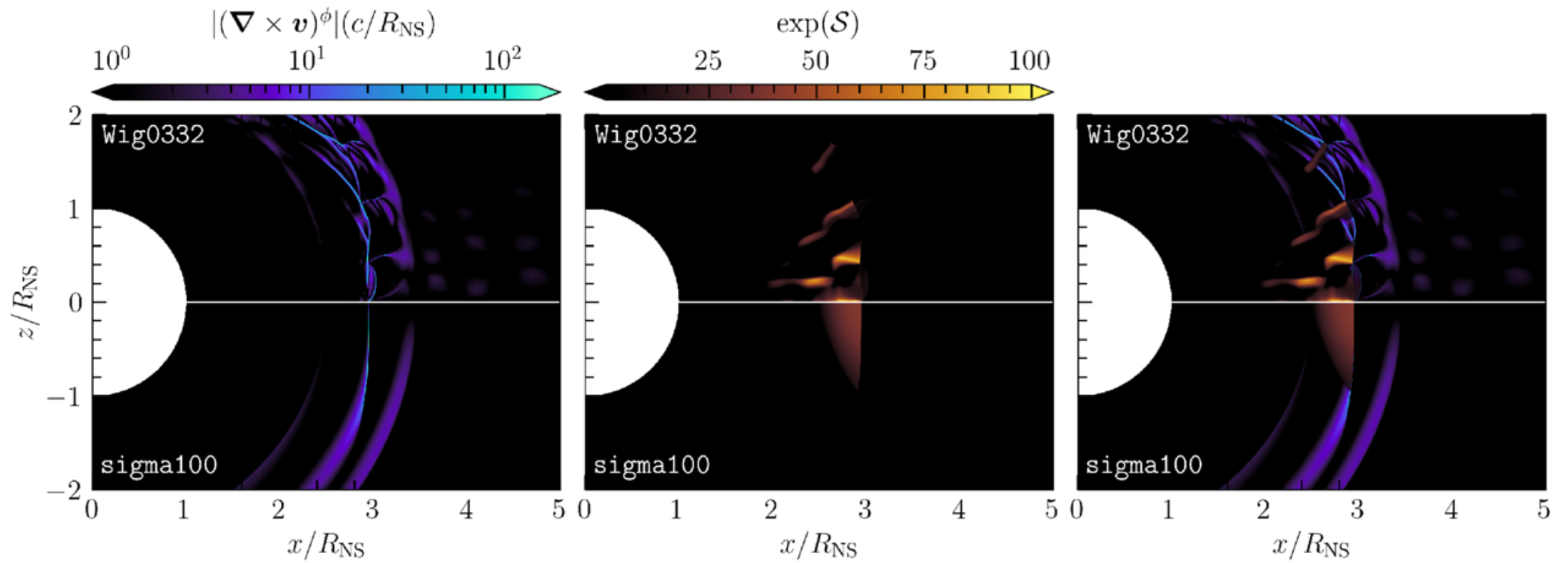
Figure 10. from Michael P. Grehan et al 2026 Astrophys. J. 1005 doi:10.3847/1538-4357/ae633a https://dx.doi.org/10.3847/1538-4357/ae633a © 2026. The Author(s). Published by the American Astronomical Society.
