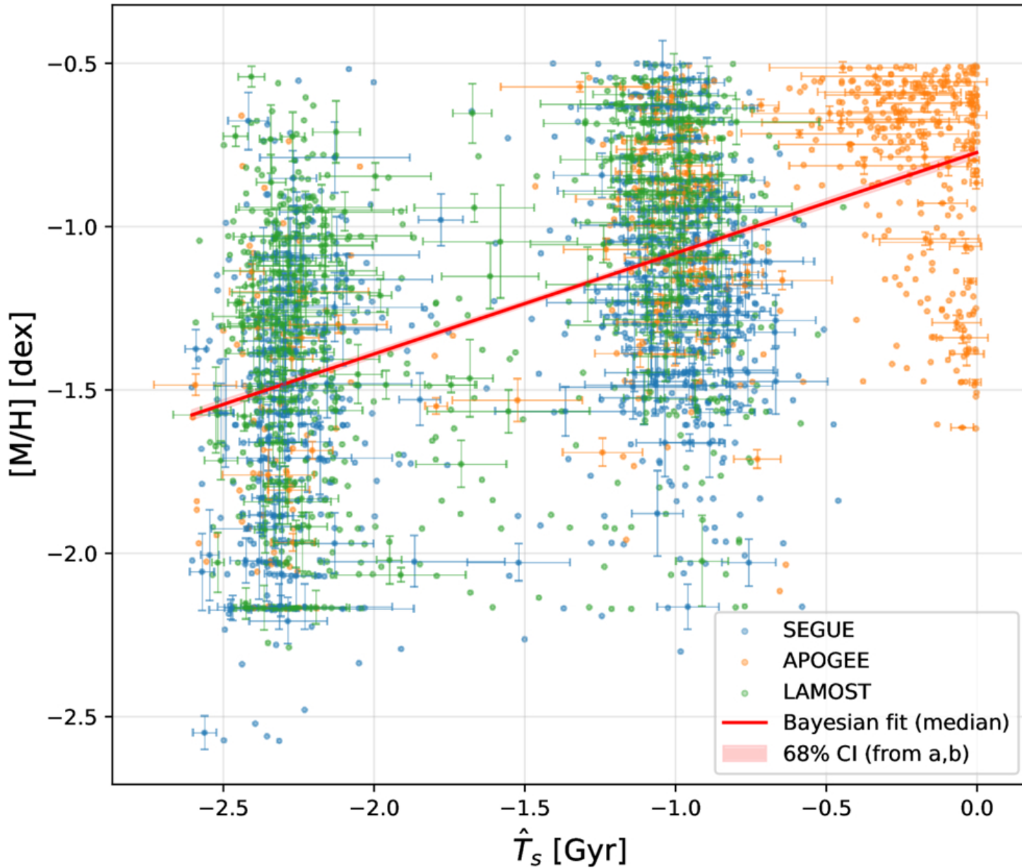
Figure 4. from Jian Zhang et al 2026 Astrophys. J. 1003 doi:10.3847/1538-4357/ae6327 https://dx.doi.org/10.3847/1538-4357/ae6327 © 2026. The Author(s). Published by the American Astronomical Society.
