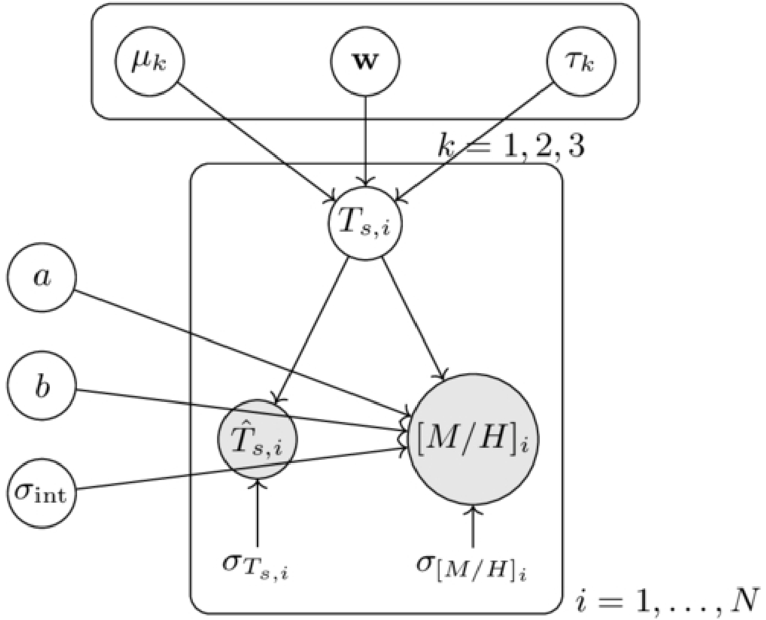
Figure 3. from Jian Zhang et al 2026 Astrophys. J. 1003 doi:10.3847/1538-4357/ae6327 https://dx.doi.org/10.3847/1538-4357/ae6327 © 2026. The Author(s). Published by the American Astronomical Society.
