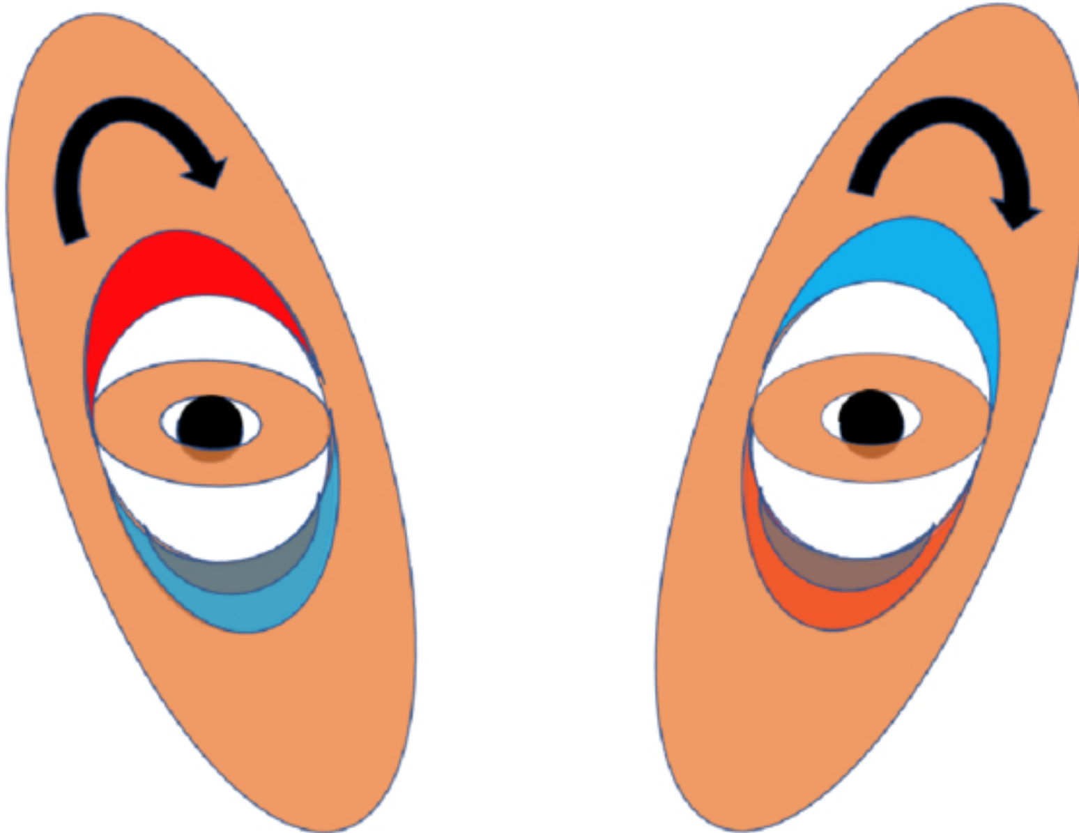
Figure 17. from William Sargent and Daniel R. Wilkins 2026 Astrophys. J. 1004 doi:10.3847/1538-4357/ae6325 https://dx.doi.org/10.3847/1538-4357/ae6325 © 2026. The Author(s). Published by the American Astronomical Society.
