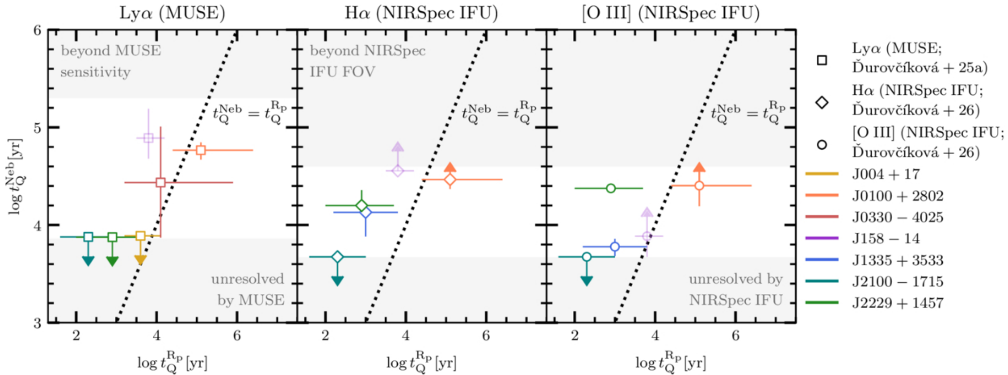
Figure 8. from Dominika urovíková et al 2026 Astrophys. J. 1003 doi:10.3847/1538-4357/ae626b https://dx.doi.org/10.3847/1538-4357/ae626b © 2026. The Author(s). Published by the American Astronomical Society.
