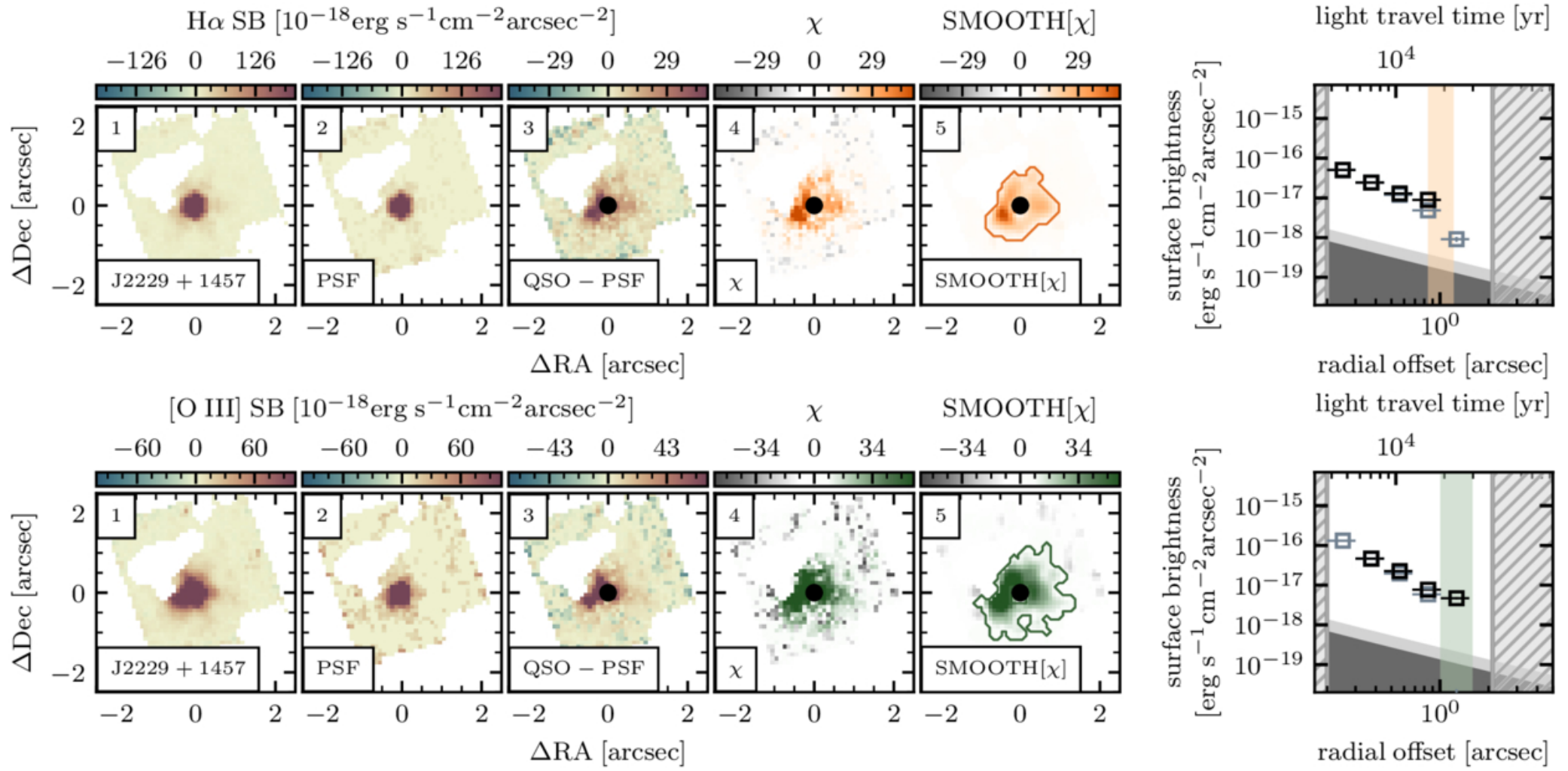
Figure 6. from Dominika urovíková et al 2026 Astrophys. J. 1003 doi:10.3847/1538-4357/ae626b https://dx.doi.org/10.3847/1538-4357/ae626b © 2026. The Author(s). Published by the American Astronomical Society.
