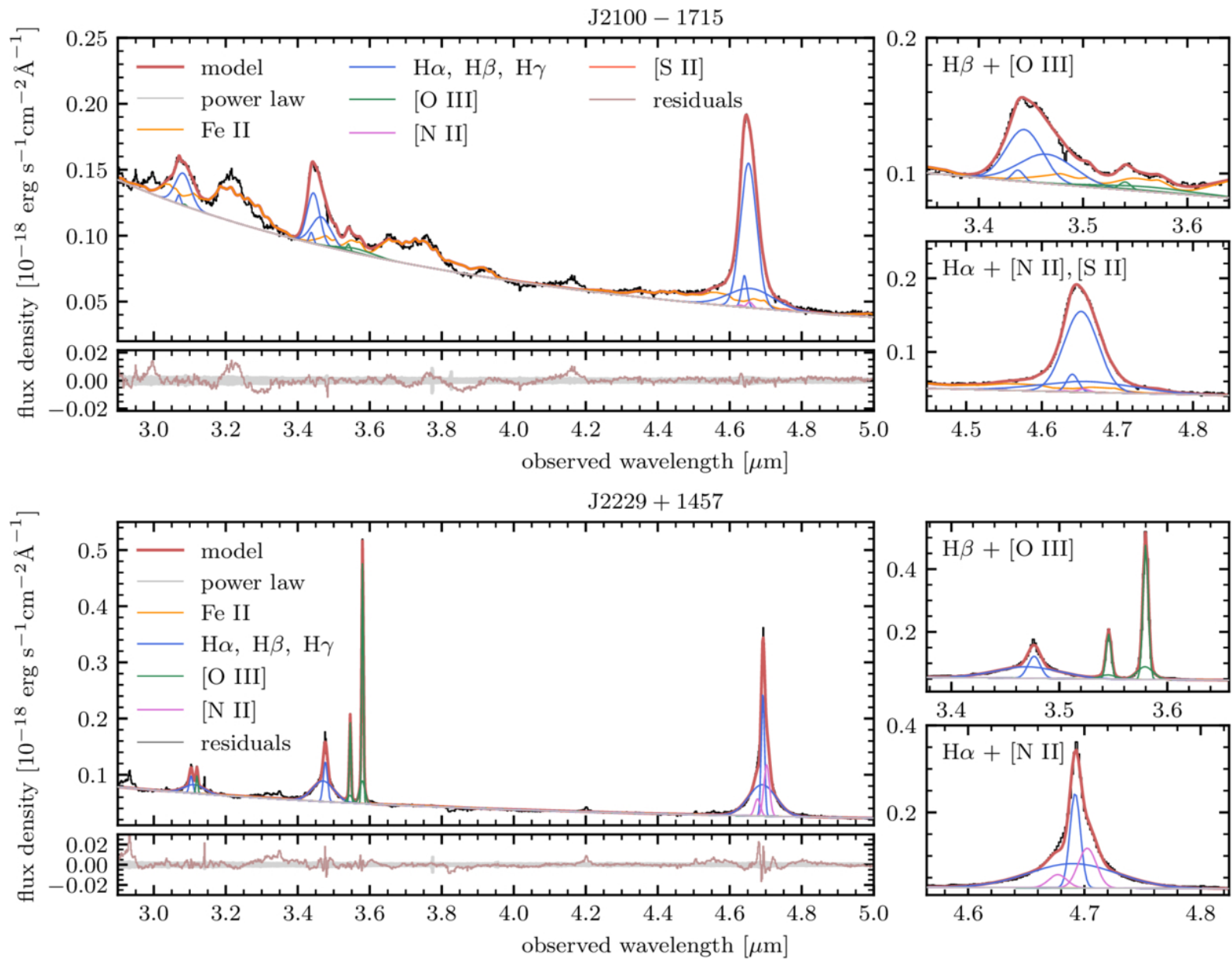
Figure 1. from Dominika urovíková et al 2026 Astrophys. J. 1003 doi:10.3847/1538-4357/ae626b https://dx.doi.org/10.3847/1538-4357/ae626b © 2026. The Author(s). Published by the American Astronomical Society.
