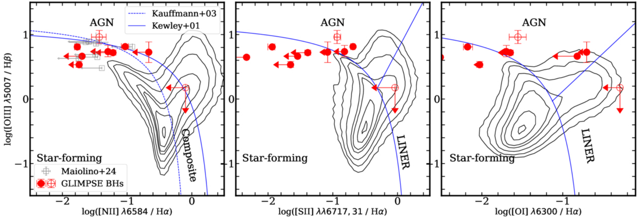
Figure 5. from Qinyue Fei et al 2026 Astrophys. J. 1003 doi:10.3847/1538-4357/ae6248 https://dx.doi.org/10.3847/1538-4357/ae6248 © 2026. The Author(s). Published by the American Astronomical Society.
