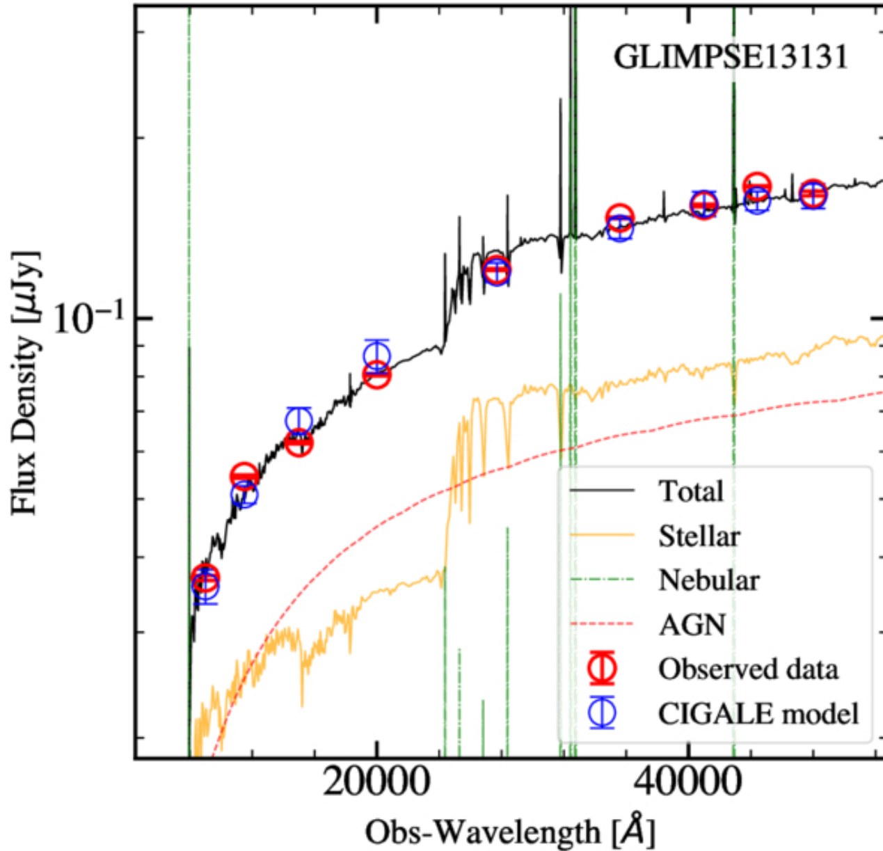
Figure 3. from Qinyue Fei et al 2026 Astrophys. J. 1003 doi:10.3847/1538-4357/ae6248 https://dx.doi.org/10.3847/1538-4357/ae6248 © 2026. The Author(s). Published by the American Astronomical Society.
