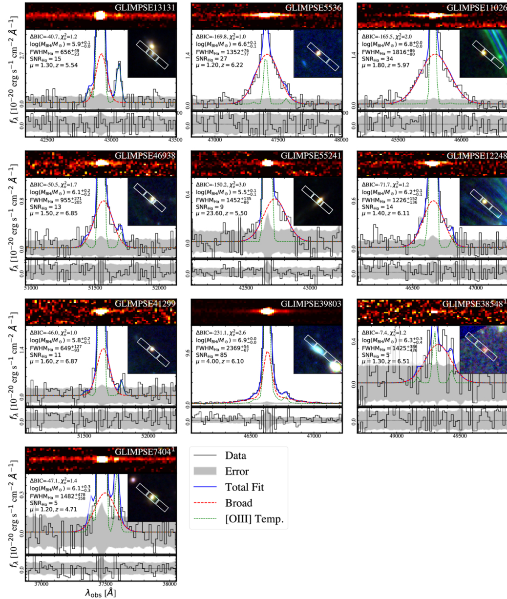
Figure 2. from Qinyue Fei et al 2026 Astrophys. J. 1003 doi:10.3847/1538-4357/ae6248 https://dx.doi.org/10.3847/1538-4357/ae6248 © 2026. The Author(s). Published by the American Astronomical Society.
