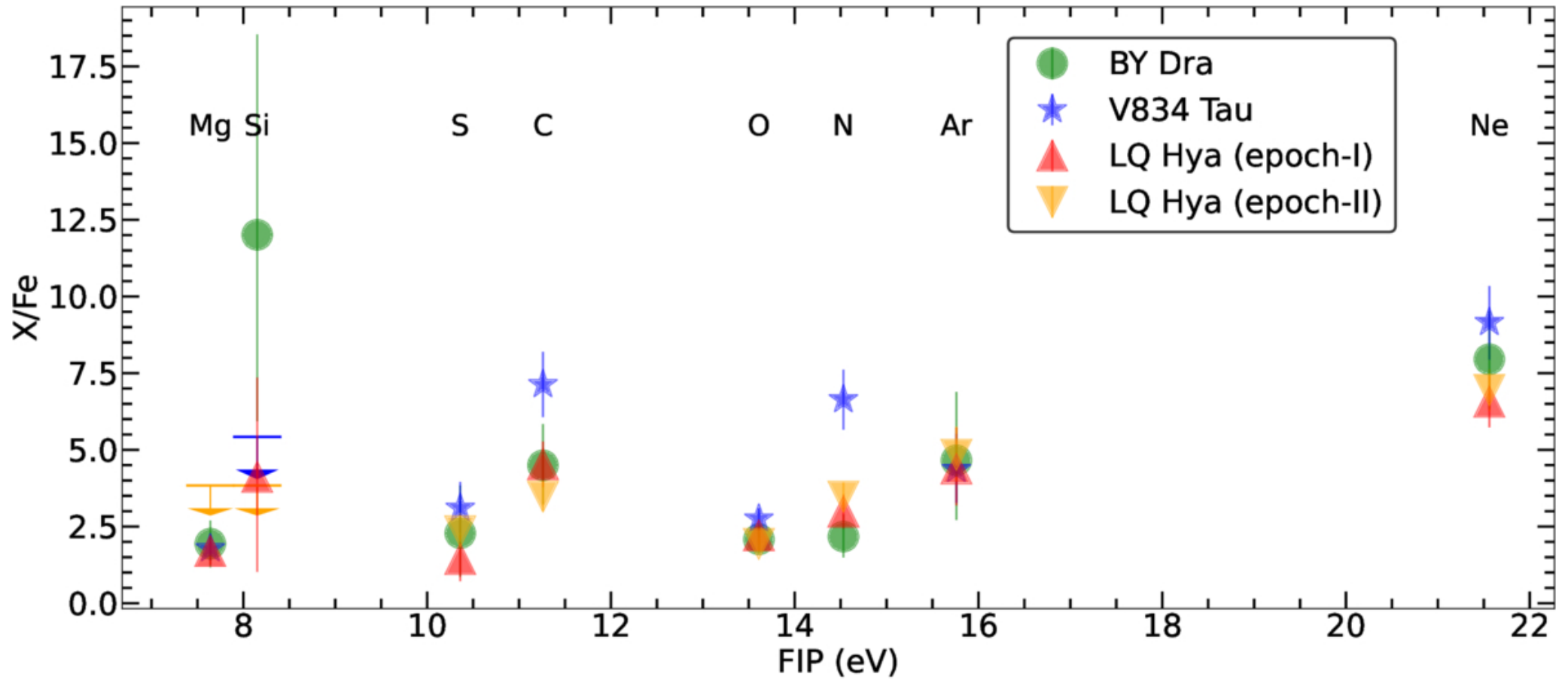
Figure 5. from Gurpreet Singh et al 2026 Astrophys. J. 1003 doi:10.3847/1538-4357/ae61a4 https://dx.doi.org/10.3847/1538-4357/ae61a4 © 2026. The Author(s). Published by the American Astronomical Society.
