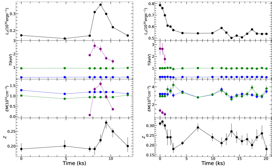
Figure 3. from Gurpreet Singh et al 2026 Astrophys. J. 1003 doi:10.3847/1538-4357/ae61a4 https://dx.doi.org/10.3847/1538-4357/ae61a4 © 2026. The Author(s). Published by the American Astronomical Society.
