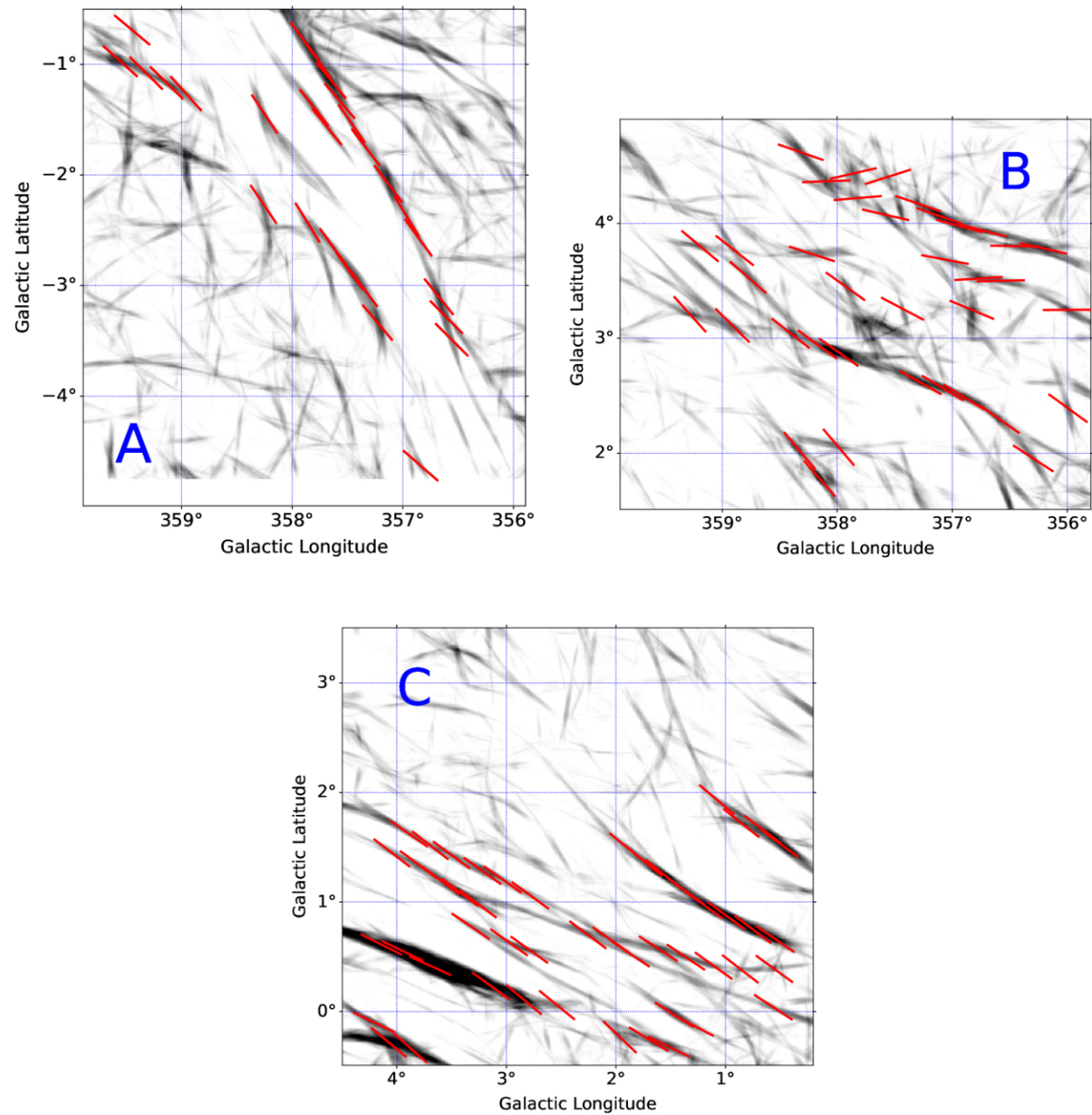
Figure 9. from Gabriel A. P. Franco et al 2026 Astrophys. J. 1004 doi:10.3847/1538-4357/ae610c https://dx.doi.org/10.3847/1538-4357/ae610c © 2026. The Author(s). Published by the American Astronomical Society.
