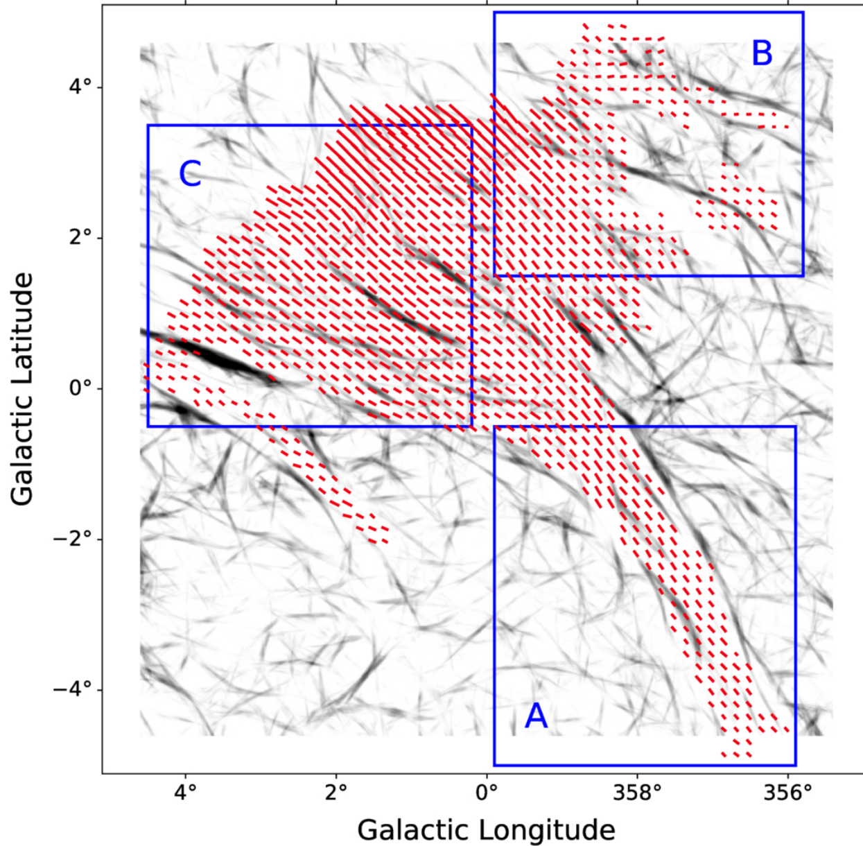
Figure 8. from Gabriel A. P. Franco et al 2026 Astrophys. J. 1004 doi:10.3847/1538-4357/ae610c https://dx.doi.org/10.3847/1538-4357/ae610c © 2026. The Author(s). Published by the American Astronomical Society.
