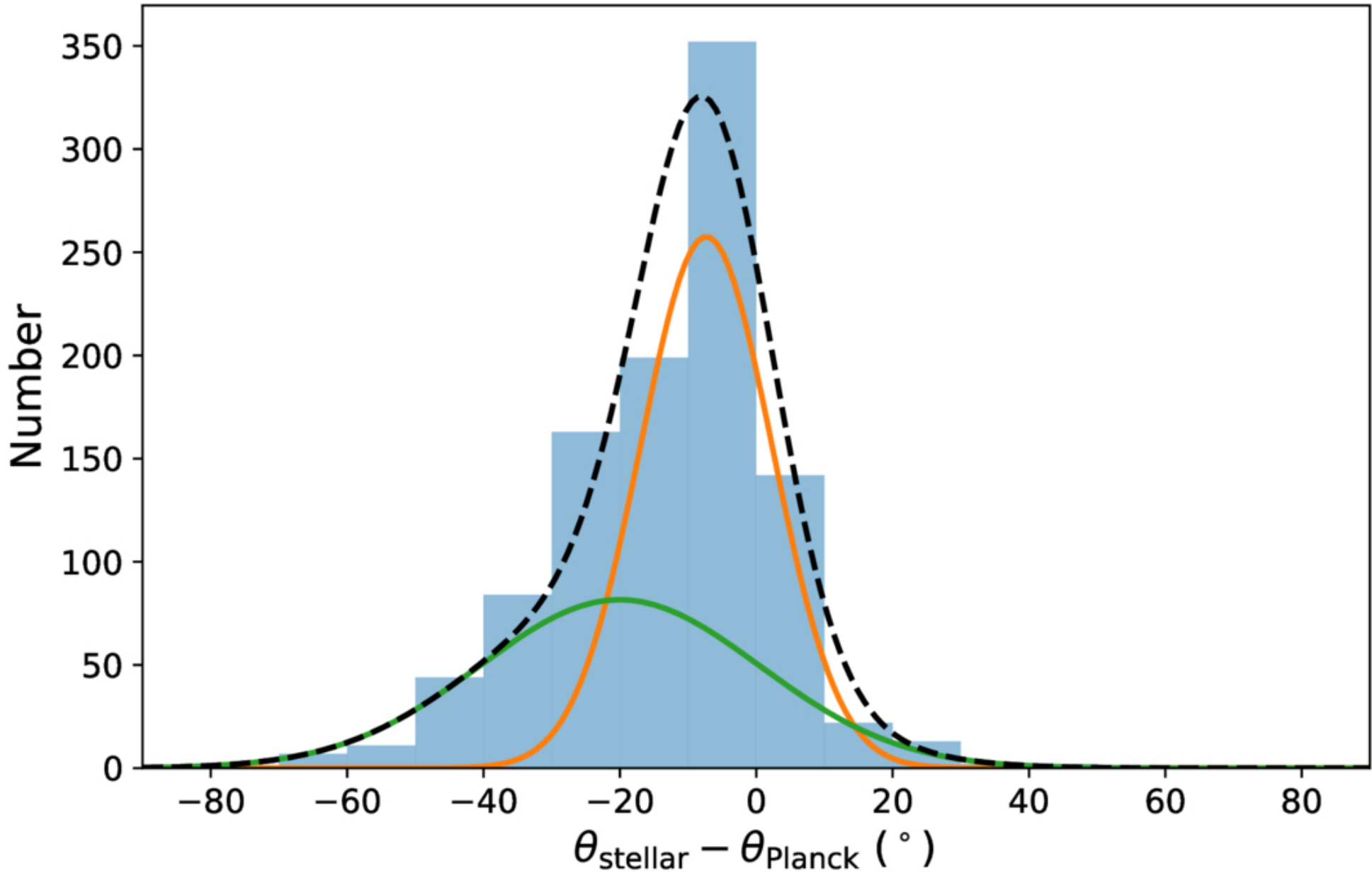
Figure 7. from Gabriel A. P. Franco et al 2026 Astrophys. J. 1004 doi:10.3847/1538-4357/ae610c https://dx.doi.org/10.3847/1538-4357/ae610c © 2026. The Author(s). Published by the American Astronomical Society.
