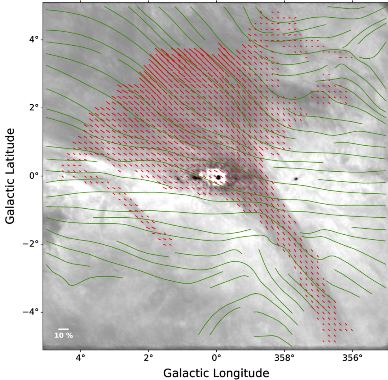
Figure 6. from Gabriel A. P. Franco et al 2026 Astrophys. J. 1004 doi:10.3847/1538-4357/ae610c https://dx.doi.org/10.3847/1538-4357/ae610c © 2026. The Author(s). Published by the American Astronomical Society.
