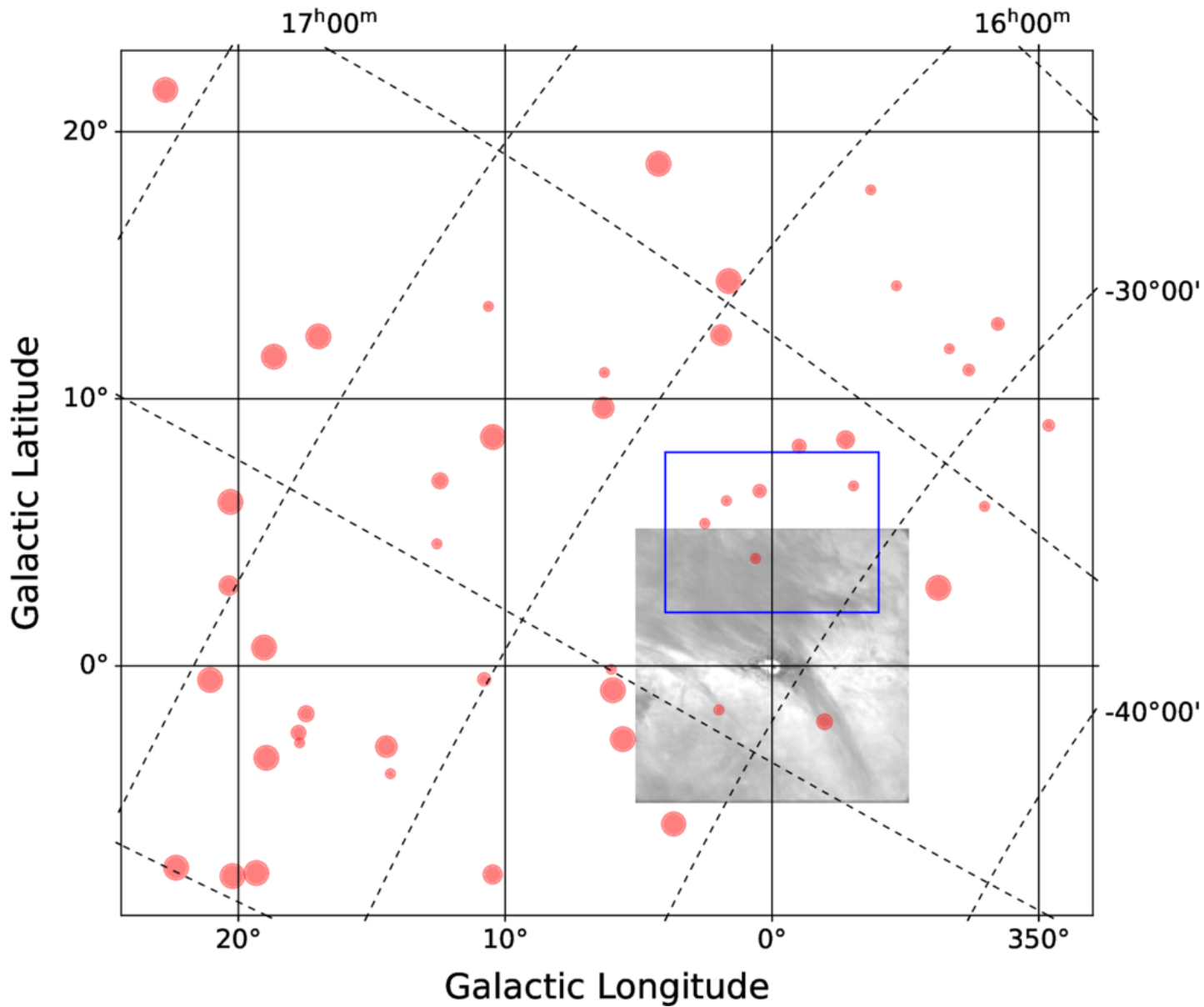
Figure 4. from Gabriel A. P. Franco et al 2026 Astrophys. J. 1004 doi:10.3847/1538-4357/ae610c https://dx.doi.org/10.3847/1538-4357/ae610c © 2026. The Author(s). Published by the American Astronomical Society.
