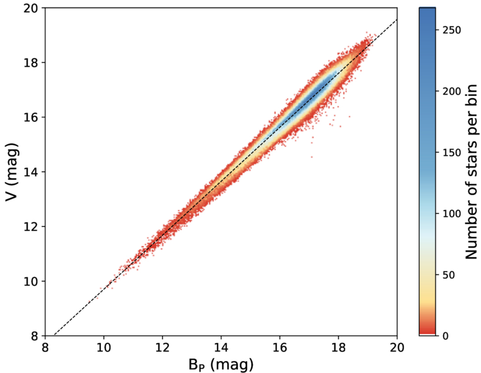
Figure 2. from Gabriel A. P. Franco et al 2026 Astrophys. J. 1004 doi:10.3847/1538-4357/ae610c https://dx.doi.org/10.3847/1538-4357/ae610c © 2026. The Author(s). Published by the American Astronomical Society.
