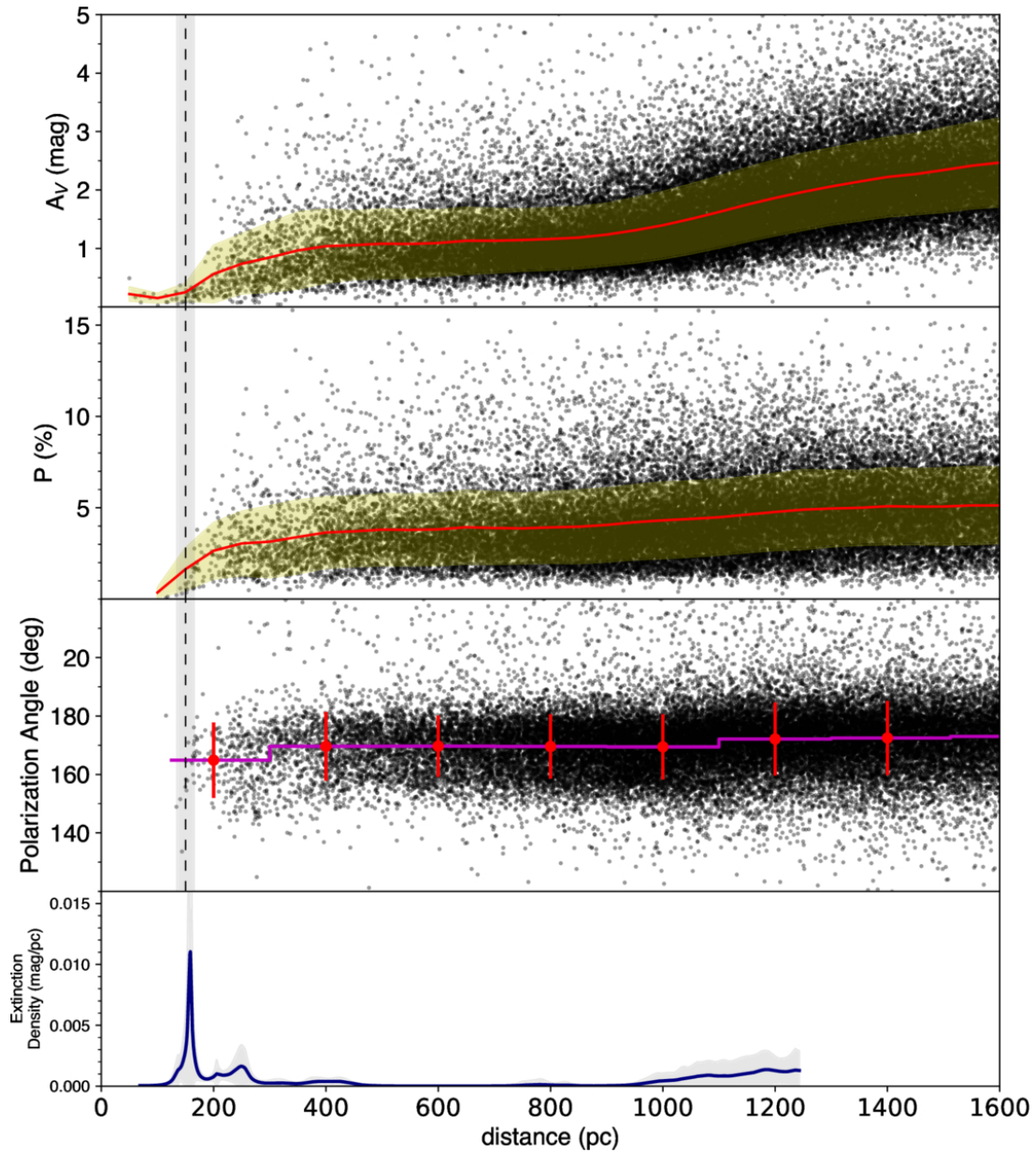
Figure 11. from Gabriel A. P. Franco et al 2026 Astrophys. J. 1004 doi:10.3847/1538-4357/ae610c https://dx.doi.org/10.3847/1538-4357/ae610c © 2026. The Author(s). Published by the American Astronomical Society.
