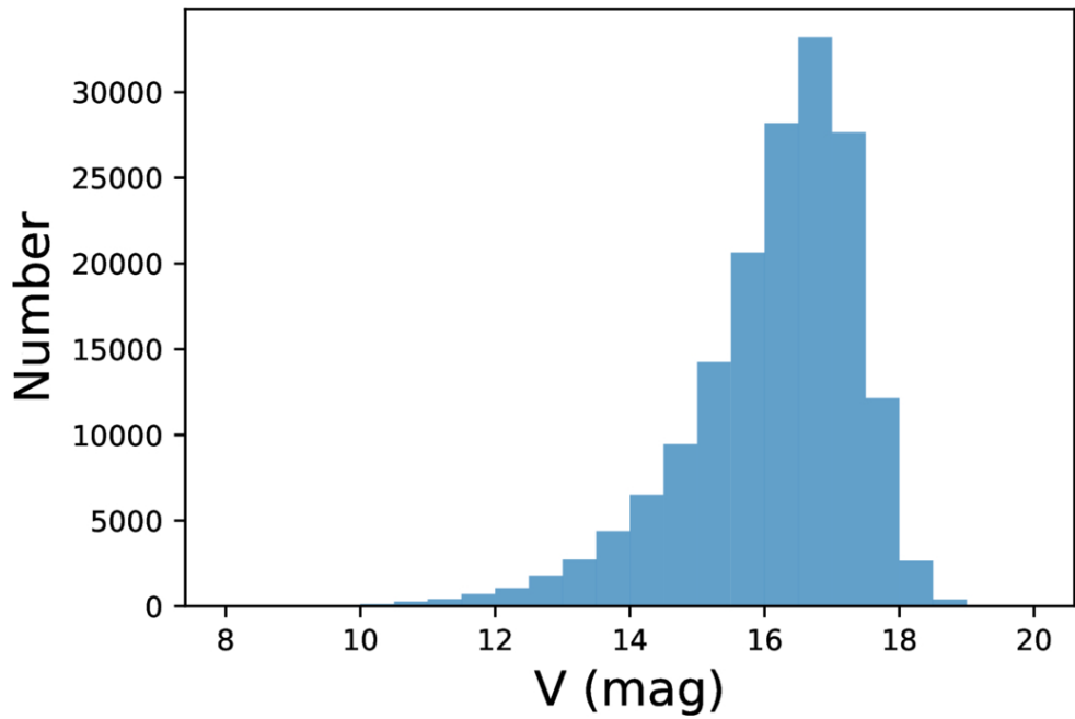
Figure 1. from Gabriel A. P. Franco et al 2026 Astrophys. J. 1004 doi:10.3847/1538-4357/ae610c https://dx.doi.org/10.3847/1538-4357/ae610c © 2026. The Author(s). Published by the American Astronomical Society.
