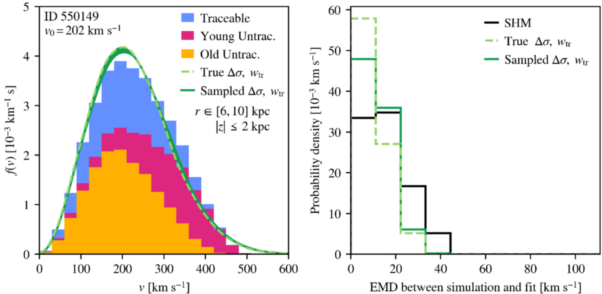
Figure 7. from Tal Shpigel et al 2026 Astrophys. J. 1003 doi:10.3847/1538-4357/ae60fd https://dx.doi.org/10.3847/1538-4357/ae60fd © 2026. The Author(s). Published by the American Astronomical Society.
