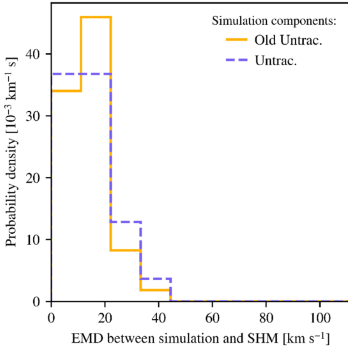
Figure 3. from Tal Shpigel et al 2026 Astrophys. J. 1003 doi:10.3847/1538-4357/ae60fd https://dx.doi.org/10.3847/1538-4357/ae60fd © 2026. The Author(s). Published by the American Astronomical Society.
