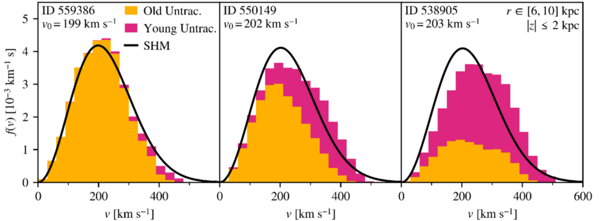
Figure 2. from Tal Shpigel et al 2026 Astrophys. J. 1003 doi:10.3847/1538-4357/ae60fd https://dx.doi.org/10.3847/1538-4357/ae60fd © 2026. The Author(s). Published by the American Astronomical Society.
