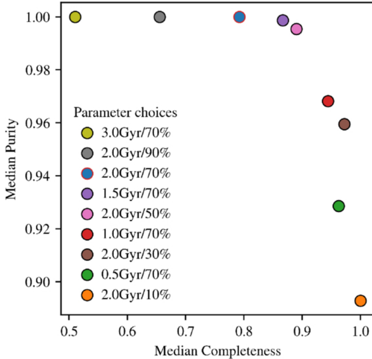
Figure A2. from Tal Shpigel et al 2026 Astrophys. J. 1003 doi:10.3847/1538-4357/ae60fd https://dx.doi.org/10.3847/1538-4357/ae60fd © 2026. The Author(s). Published by the American Astronomical Society.
