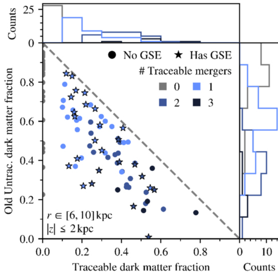
Figure 1. from Tal Shpigel et al 2026 Astrophys. J. 1003 doi:10.3847/1538-4357/ae60fd https://dx.doi.org/10.3847/1538-4357/ae60fd © 2026. The Author(s). Published by the American Astronomical Society.
