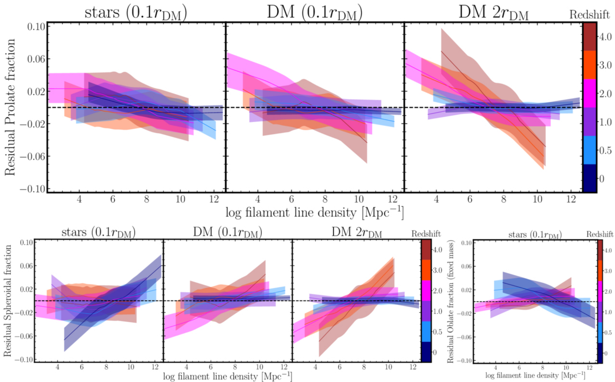
Figure 7. from Farhanul Hasan et al 2026 Astrophys. J. 1004 doi:10.3847/1538-4357/ae60f9 https://dx.doi.org/10.3847/1538-4357/ae60f9 © 2026. The Author(s). Published by the American Astronomical Society.
